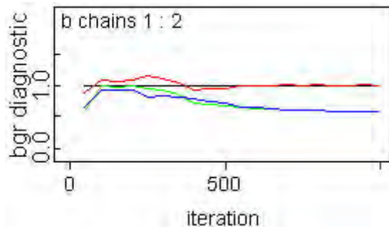
• Figure 4-39. BGR diagnostic for “b” parameter, indicating convergence.
