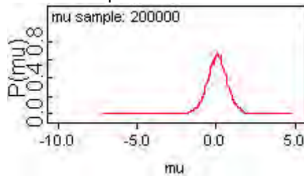
• Figure 4-65. Posterior distribution of \mu in Example 23.
