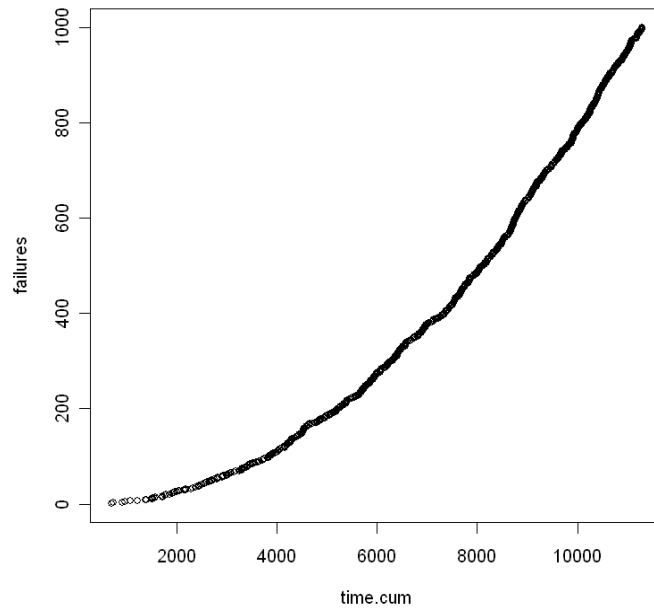
• Figure 4-75 Cumulative failure plot for 1,000 times simulated from power-law process with shape parameter of 2, illustrating increasing ROCOF
