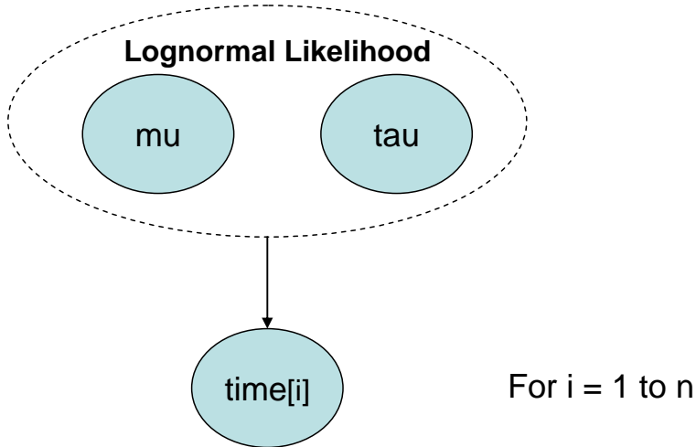
• Figure 4-64. DAG representing Script 29.
