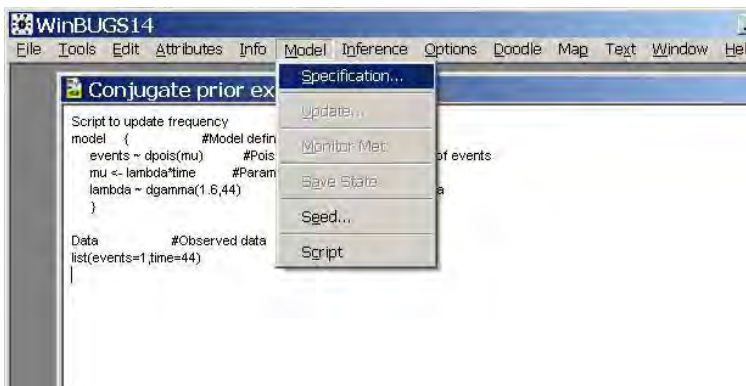
Figure C.2: Checking the WinBUGS model for syntax.
