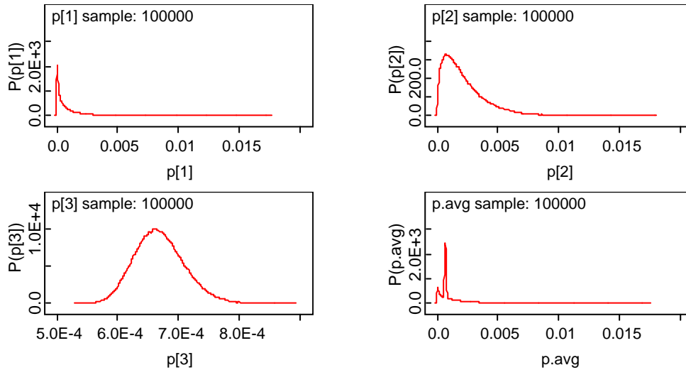
• Figure 4-120. Parameter densities for the example.
