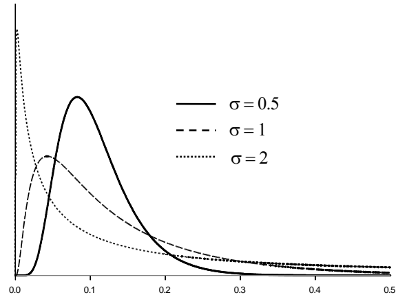
Figure B.18 Three logistic-normal densities with median = 0.1.
