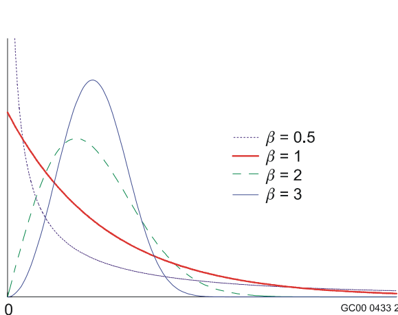
Figure B.12 Four Weibull densities, all having \theta = 0 and all having the same \alpha .
