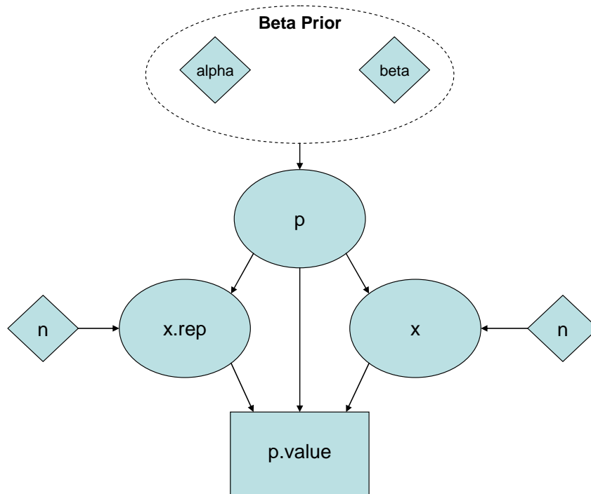
• Figure 4-15. DAG representing Script 11.
