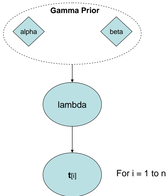
• Figure 4-10. DAG representing Script 6.
