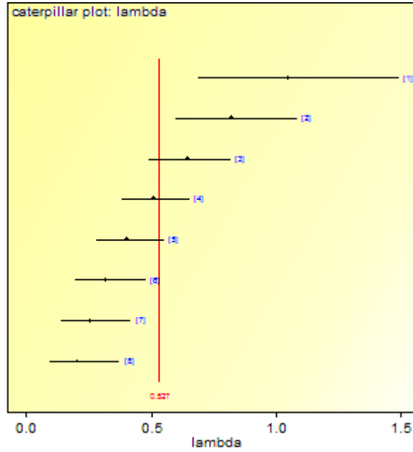
• Figure 4-41. Plot of 95% interval for lambda in each year based on a trend model in which lambda is decreasing with time.
