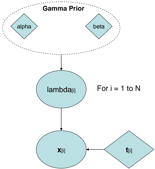
• Figure 4-23. DAG representing Script 17.
