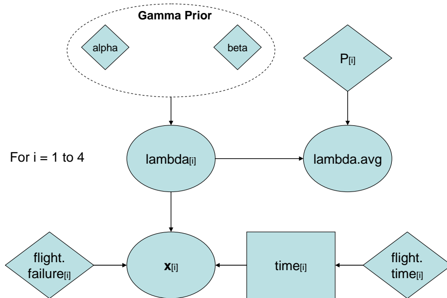
• Figure 4-98. DAG representing Script 52.
