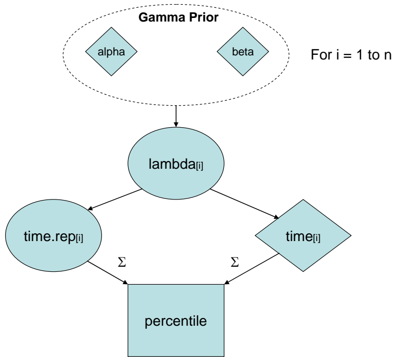
• Figure 4-25. DAG representing Script 19.
