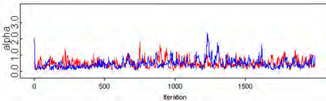
• Figure 4-43. Plot of first 2,000 values of alpha, indicating convergence.
