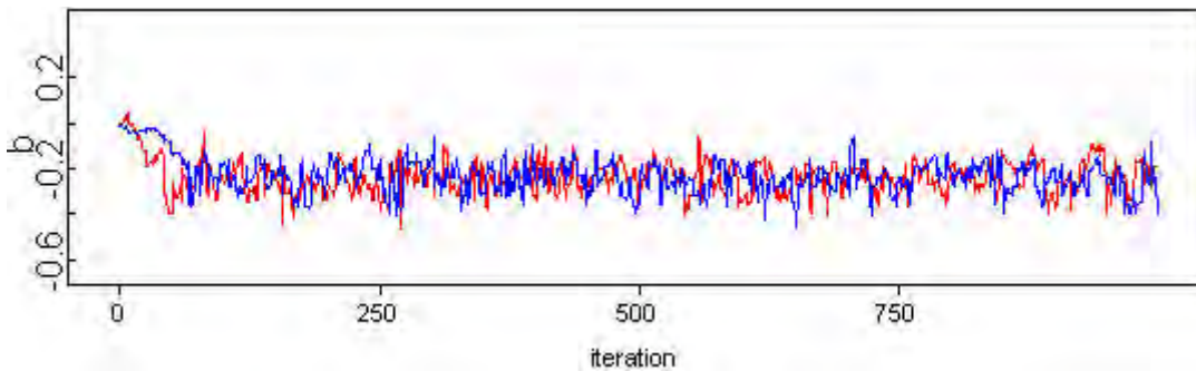
• Figure 4-37. Plot of values of first 1,000 values for “b” parameter, illustrating convergence.
