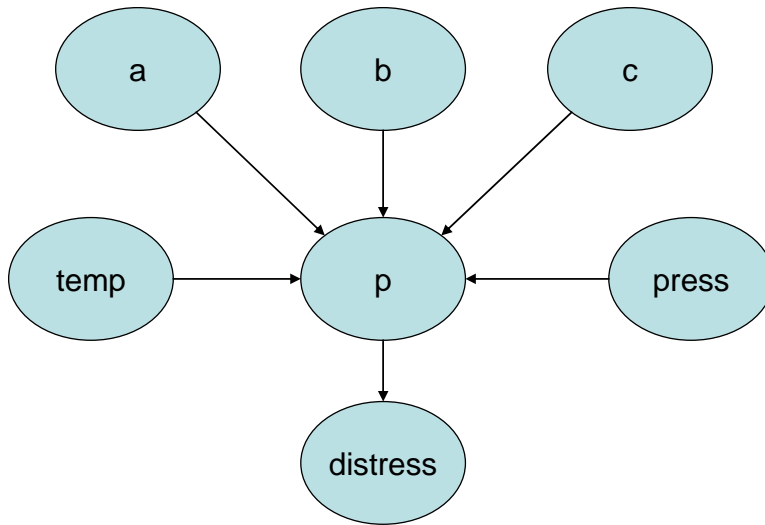
• Figure 4-92. DAG representing Script 48.
