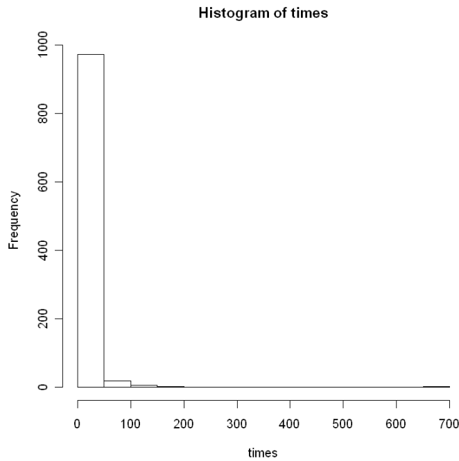
• Figure 4-76. Histogram of times between failures for simulated failure times from power-law process with increasing ROCOF.
