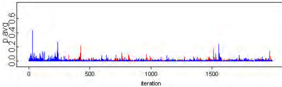
• Figure 4-47. Plot of first 2,000 values of p.avg, indicating convergence.
