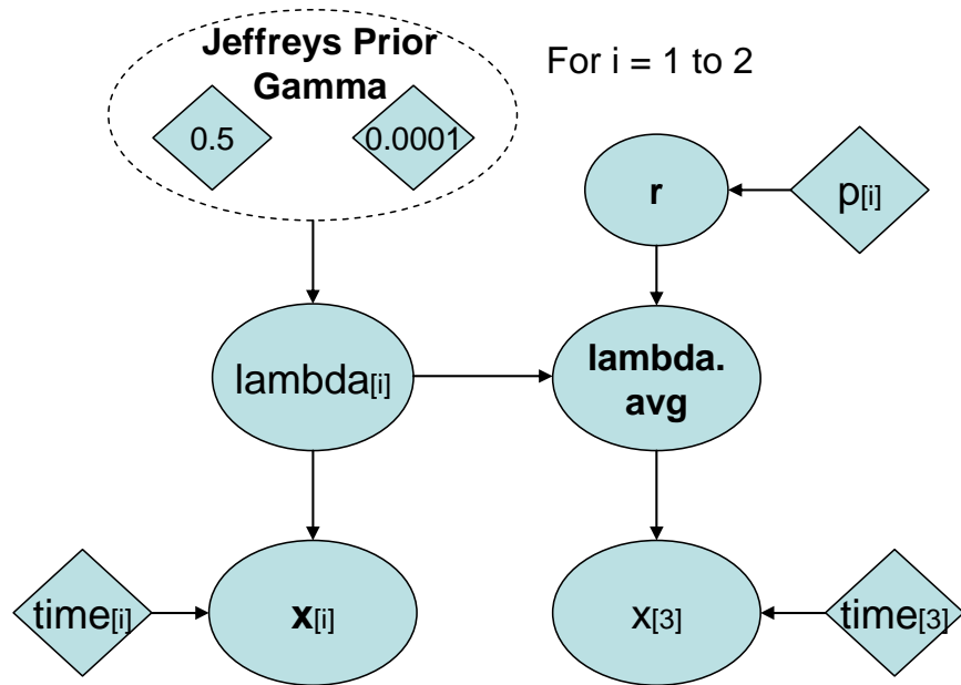
• Figure 4-114. DAG representing Script 63, Script 65, and Script 67.
