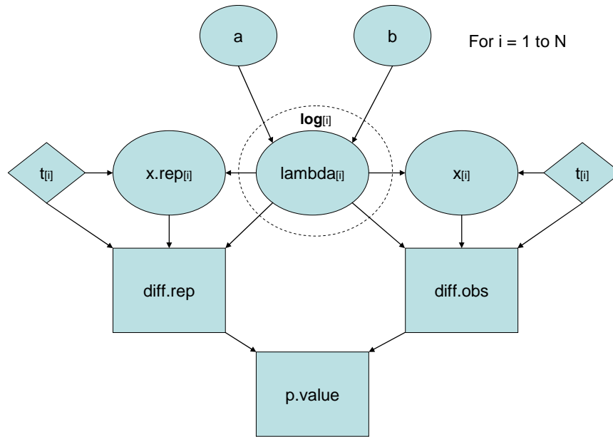
• Figure 4-35. DAG representing Script 22.
