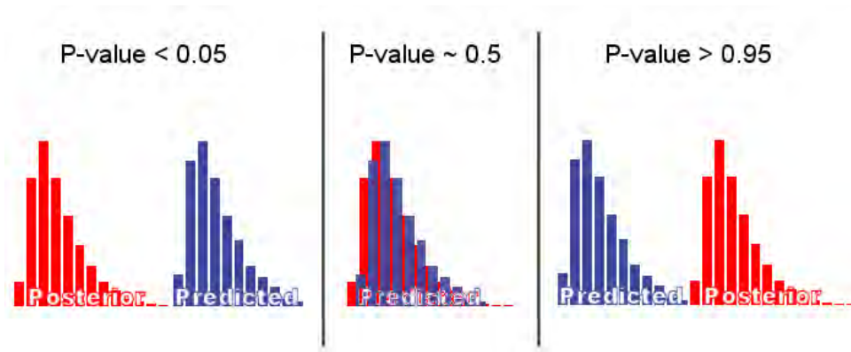
• Figure 4-14. Illustration of the Bayesian p.value calculation used to test on prior, posterior, or model validity.
