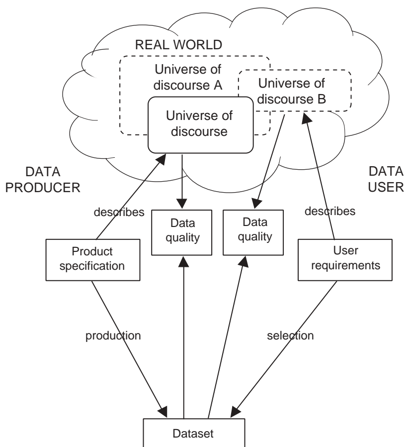
Figure B.1 — The framework provided by data quality concepts
