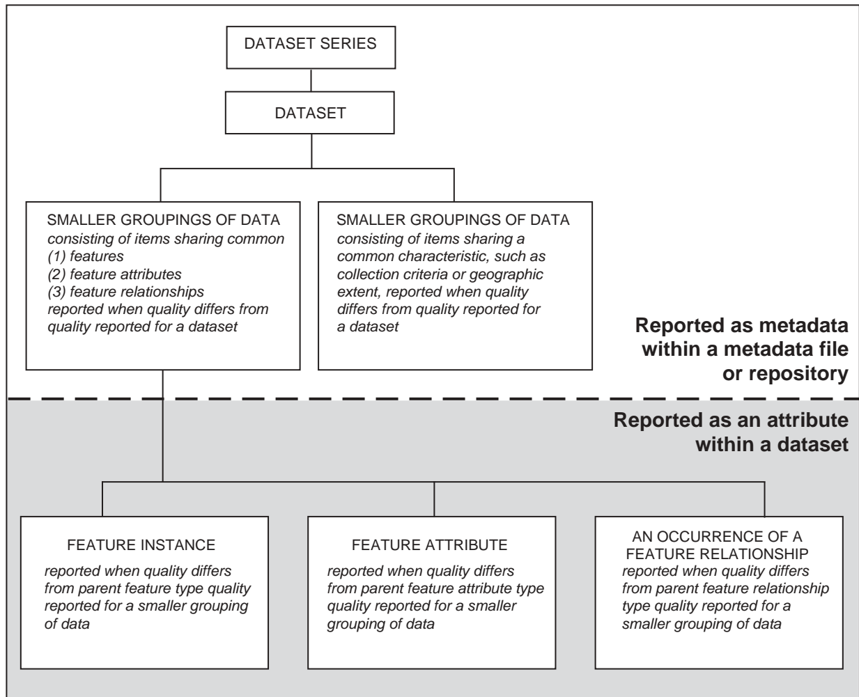
Figure B.2 — A suggested method of reporting quantitative quality information as metadata
