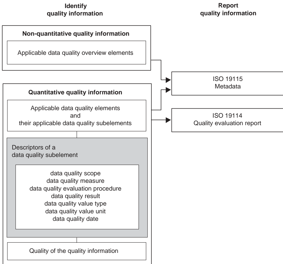
Figure 1 — An overview of data quality information
