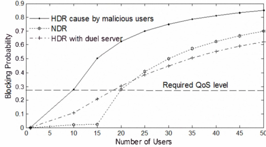
Fig. 5. Queuing comparisons for the QoS requirements
