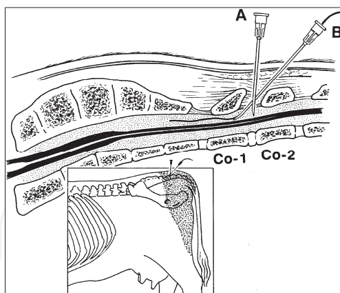
Fig. 1. For caudal and epidural anesthesia in cattle the injection site used is between coxyls Co-1 and Co-2 (Modified from Thurmon et al , 1996)
