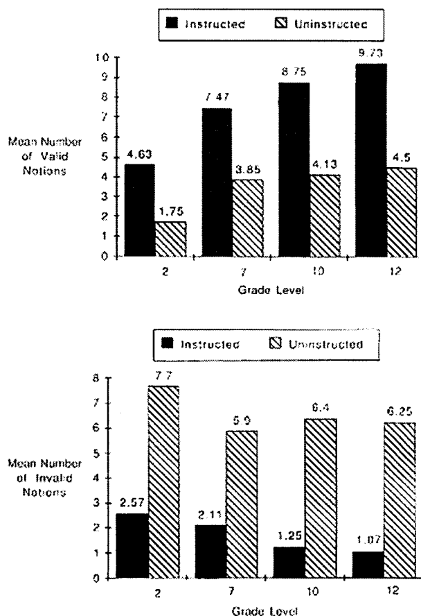
Figure 4: The number of valid and invalid notions held by Instructed and Uninstructed students in grades 2, 7, 10, and 12.
