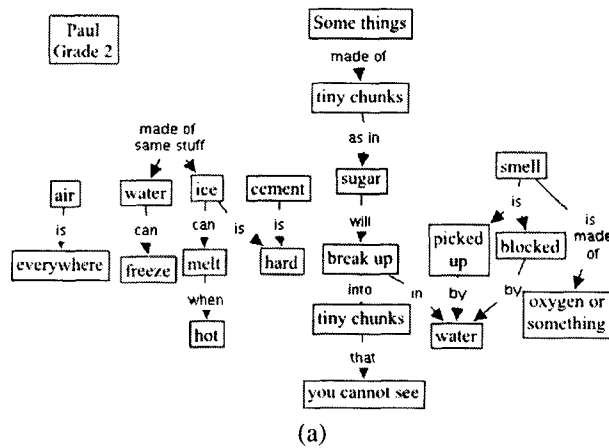
Figure 3: Two concept maps constructed from interviews with an exceptionally good Uninstructed student at the ends of grades 2 (a), and 12 (b).
